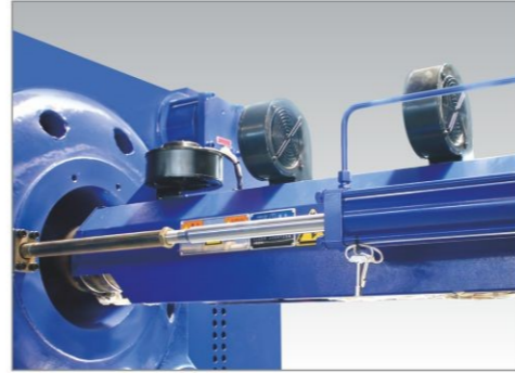
Air fan cooling equipment on the barrel, PID temperature control system.
